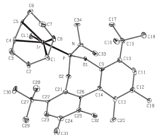
Figure 2. ORTEP representation of the structure of [Ir(cod)(L 4 )Cl]; selected bond lengths [Å] with estimated standard deviations: Ir-Cl 2.362(2), Ir-P 2.265(3), Ir-C1 2.126(9), Ir-C4 2.224(10), Ir-C5 2.232(10), Ir-C8 2.143(9), C1-C8 1.435(16), C4-C5 1.397(17).
